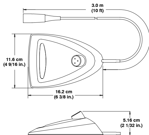
DIMENSIONS FIGURE 2
