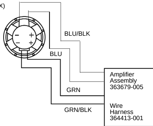
WIRE HARNESS SCHEMATIC ( 364413-001)
