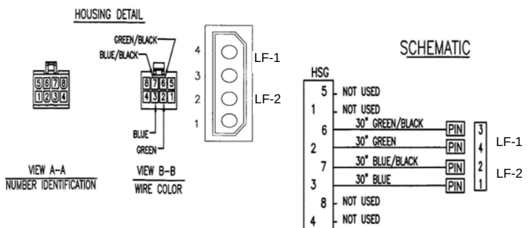
WIRE HARNESS SCHEMATIC ( 364413-001)
